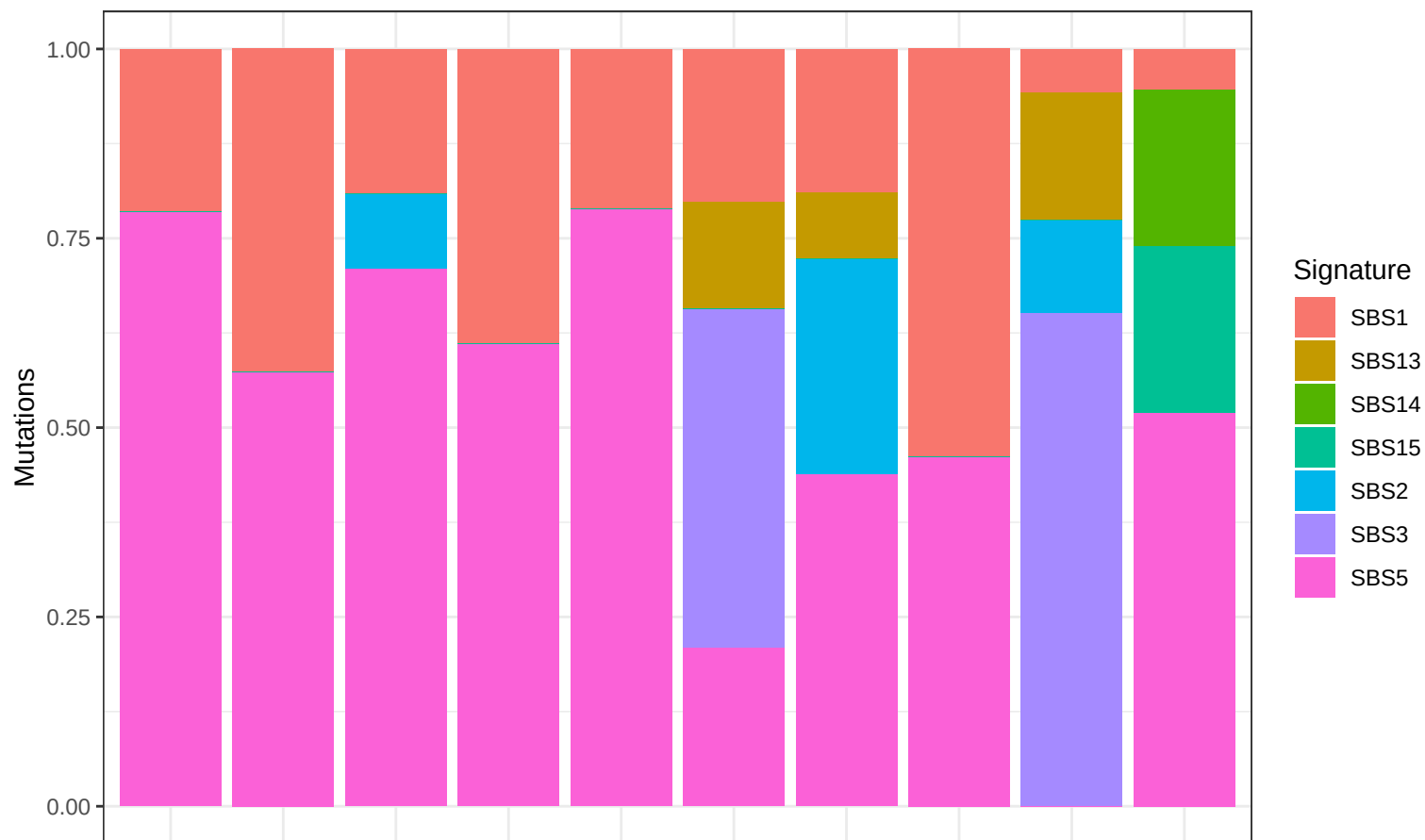
PAAD – Top 10 most mutated samples
